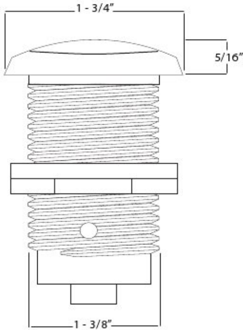
Assembly View
